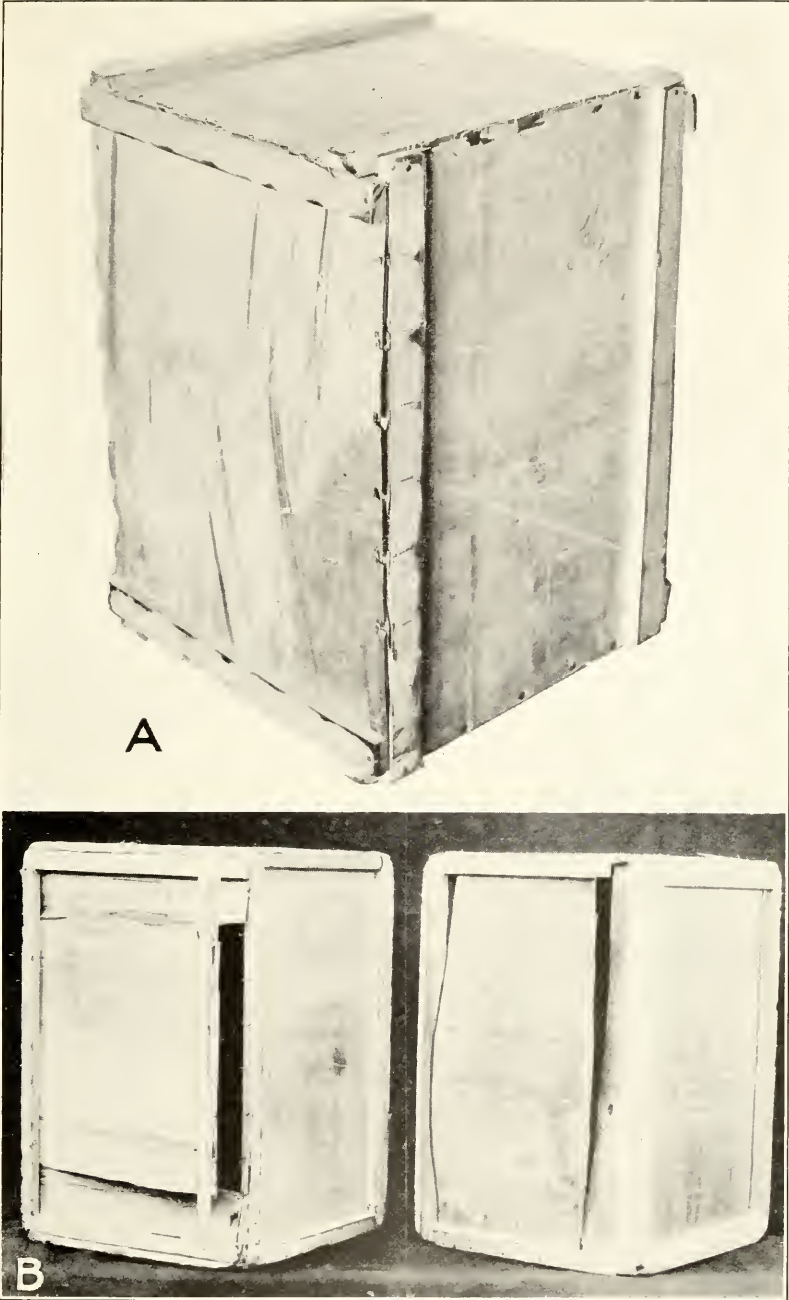
A, Characteristic failure of single cleated plywood box; B, characteristic failures of cleated plywood boxes
